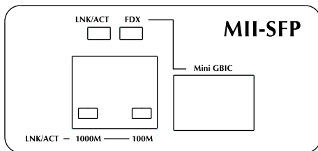
Figure 6. 1-Port 1000Base-T/Mini GBIC Module Front View
